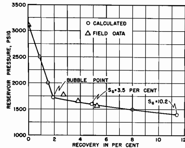
Fig. 5.4. Material balance calculations and performance, Canyon Reef reservoir, Kelly-Snyder Field.
