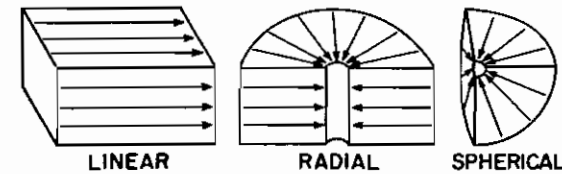
Fig. 7.1. Common flow geometries.
