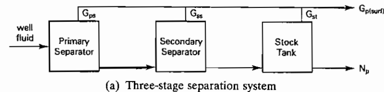
(a) Three-stage separation system
