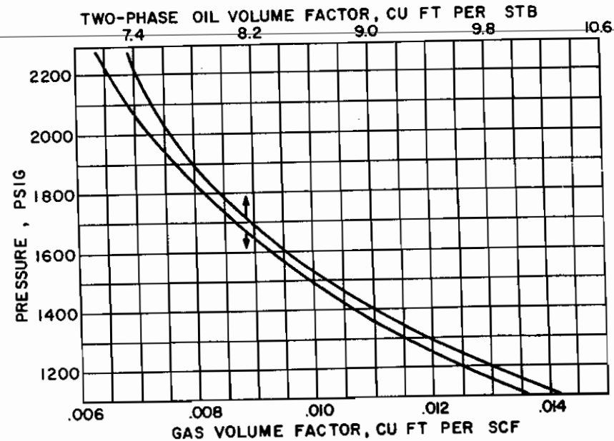
Fig. 8.4. Pressure volume relations for Conroe Field oil and original complement of dissolved gas. (After Schilthuis. 3 )
