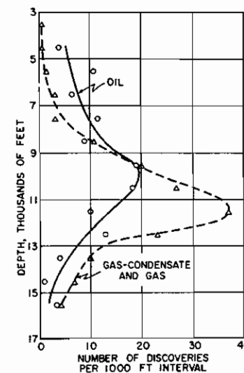
Fig. 4.1. Discovery frequency of oil and gas or gas-condensate reservoirs versus depth. For 17 parishes in southwest Louisiana, 1952–1956, inclusive. (Data from Ira Rinehart's Yearbooks . 2 )
