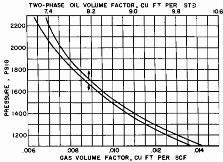
Fig. 6.2. Pressure volume relations for Conroe Field oil and original complement of dissolved gas. (After Schilthuis, 3 Trans. AIME.)
