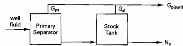
(b) Two-stage separation system
