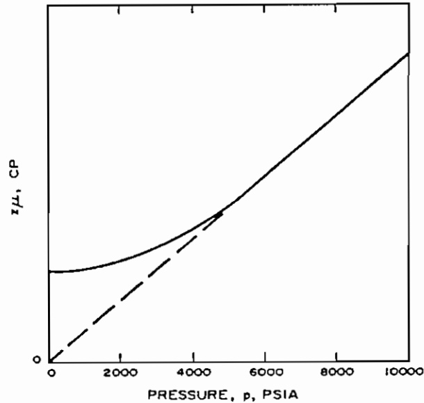
Fig. 7.4. Isothermal variation of \mu z with pressure.
