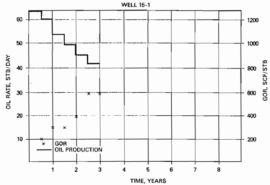
Fig. 10.6. Actual production and instantaneous GOR for history matching problem.
