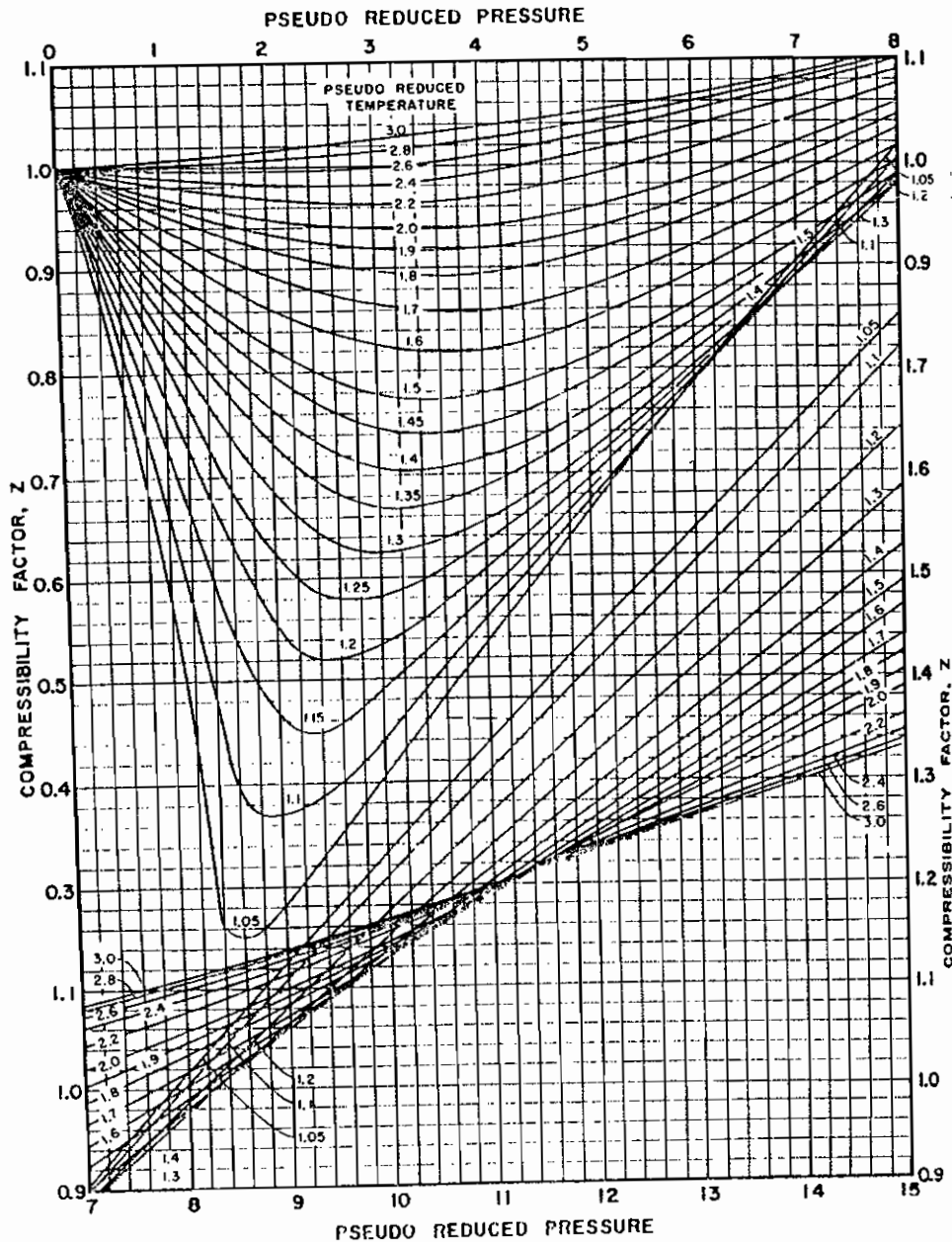
Fig. 1.5. Compressibility factors for natural gases. (After Standing and Katz, Trans. AIM. )
