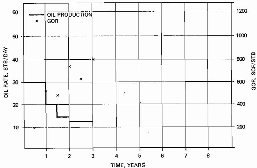
Fig. 10.18. Actual oil production and instantaneous GOR for Wells 5-6 for Problem 10.3.
