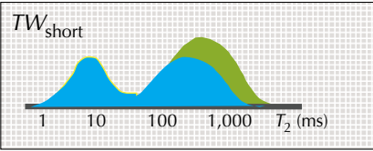
T_2 Distribution
