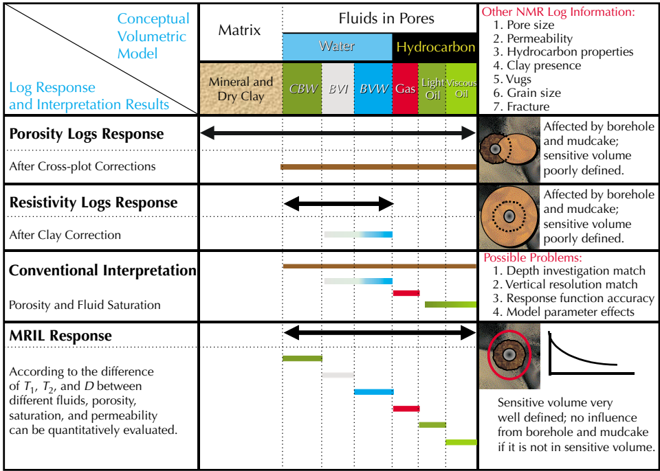
Figure 1.3 —MRIL tool responses are unique among logging tools. MRIL porosity is independent of matrix minerals, and the total response is very sensitive to fluid properties. Because of differences in relaxation times and/or diffusivity among fluids, MRIL data can be used to differentiate clay-bound water, capillary-bound water, movable water, gas, light oil, and viscous oils. Other information, such as pore size, permeability, hydrocarbon properties, vugs, fractures, and grain size, often can be extracted. In addition, because the volumes to which MRIL tools are sensitive are very well defined, borehole fluids and rugosity minimally affect MRIL measurements.
