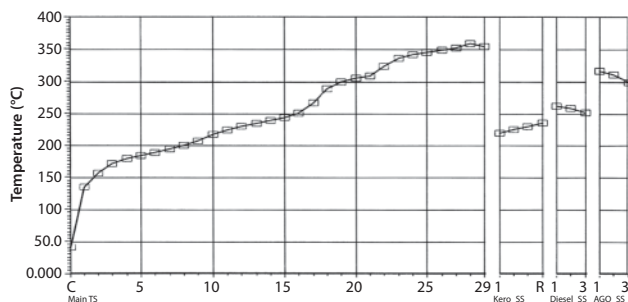
Figure 5.23 Temperature vs. tray position from top.
