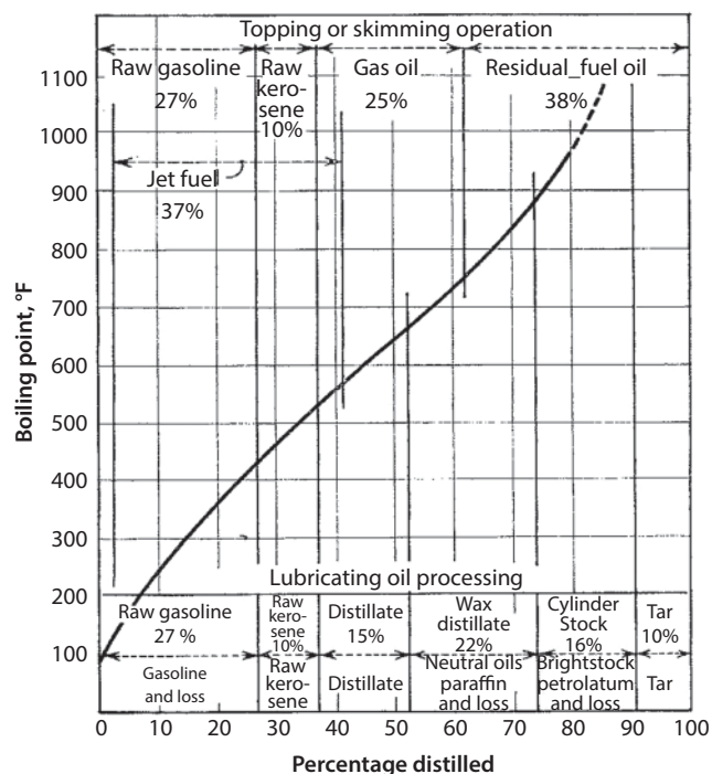
Figure 5.3 Boiling range of refinery products (31.7 °API Texas mixed-base crude oil) (Source: Nelson, W. L., Petroleum Refinery Engineering , 4 th ed., McGraw-Hill Series in Chemical Engineering, 1958).
