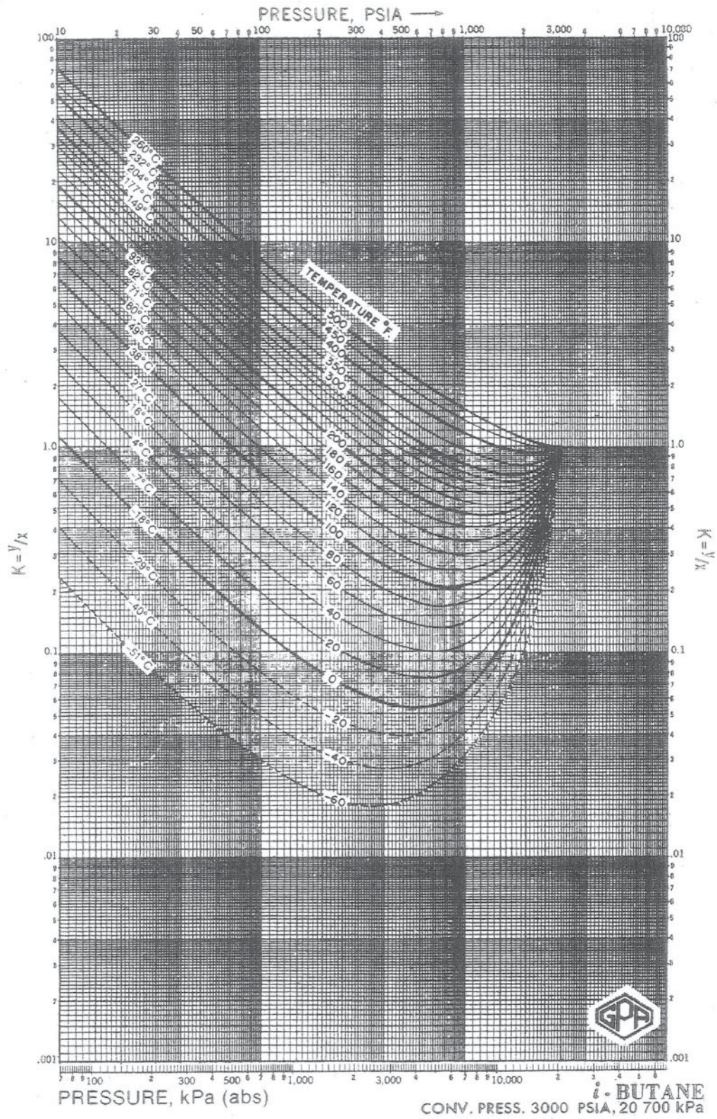
Figure A.4 Pressure vs. K for i -Butane ( i\text{-C}_4\text{H}_{10} ) at convergence pressure of 3000 psia (20,700 kPa). Used by permission, Gas Processors Suppliers Association Data Book, 12 th Ed., V. 1 and 2, (2004), Tulsa, Okla.
