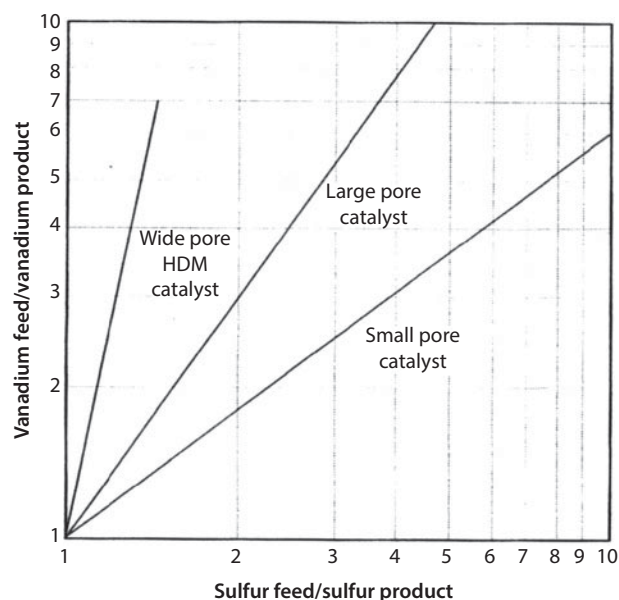
Figure 7.32 General relationship between vanadium and sulfur removal for different Co-Mo catalyst (Source: Raseev, S., Thermal and Catalytic Processes in Petroleum Refining , Marcel Dekker, New York, 2003).
