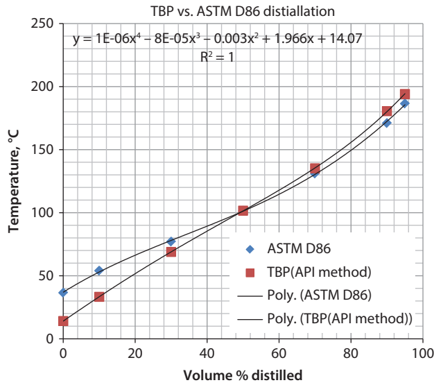
Figure 3.8a Conversion of ASTM D86 to TBP.
