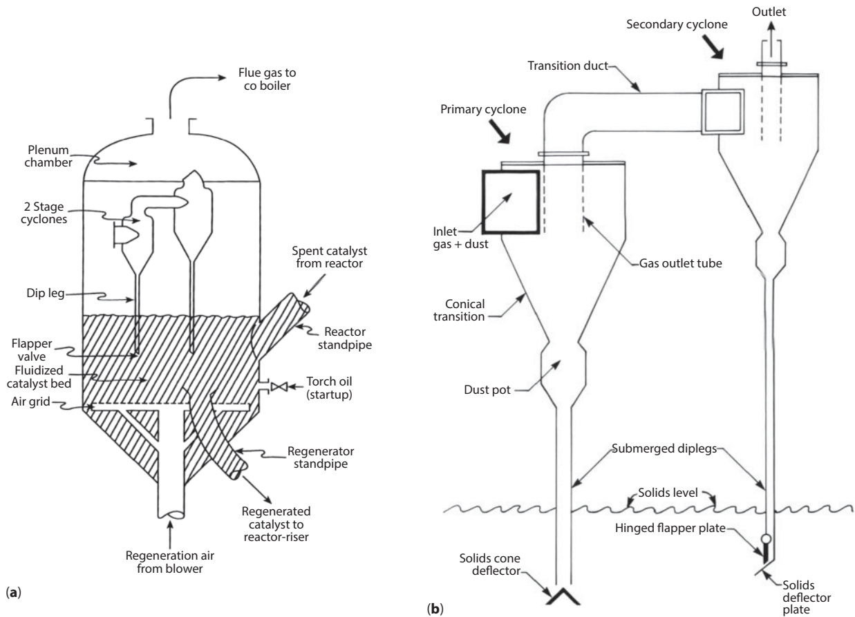
Figure 8.5 (a) FCC regenerator (Source: Gary, James, H. et al. Petroleum Refining—Technology and Economics 5 th ed., CRC Press, Taylor & Francis Group, 2007). (b) Typical two-stage cyclone (Source: Lieberman, Norman P., Troubleshooting Process Operations , 2 nd ed., PennWell Publishing Co., 1985).
