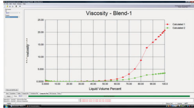
Figure 4.10 Snapshot of liquid volume (%) vs. viscosity of petroleum blend (Courtesy of Honeywell UniSim software), Honeywell (R) and UniSim (R) are registered trademarks of Honeywell International Inc.
