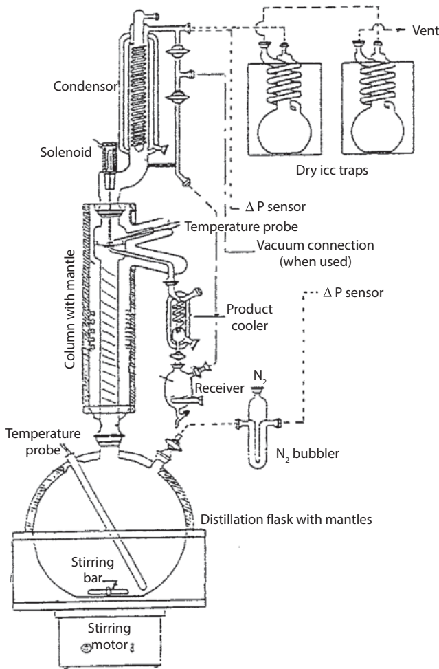
Figure 3.5 The True Boiling Point (TBP) distillation apparatus.
