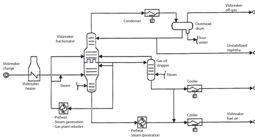
Figure 6.25 Process flow diagram of a typical visbreaker unit [9].
