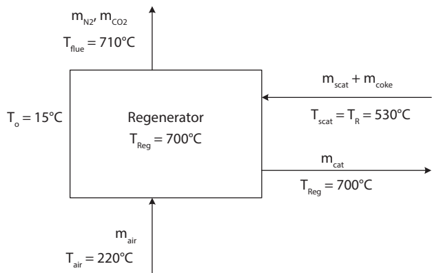
Figure 8.21 Regenerator.
