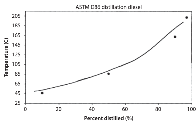
Figure 8.28 ASTM D-86 distillation for the product gasoline from debutanizer column (VALID-1) [Source: Chang, Ai-Fu., et al. (21)].
