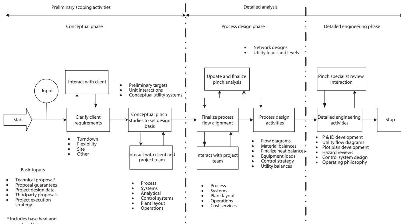
Figure 26 This new process design work process implements process integration effectively. (Source: Stephen W. Morgan, “Use Process Integration to Improve Process Designs and the Design Process”, Chemical Engineering Process, p 62, September 1992 [5]).
