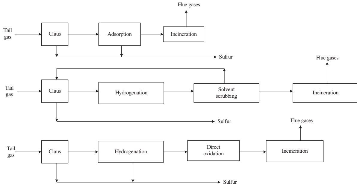
Figure 12.11 Typical Tail gas clean-up scheme [27].
