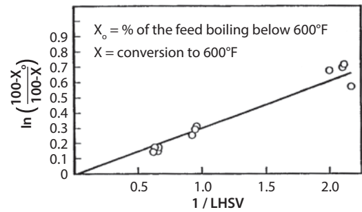
Figure 7.6 Sherzer and Gruia (Source: Hydrocracking Science and Technology , Marcel Dekker, New York 1996).
