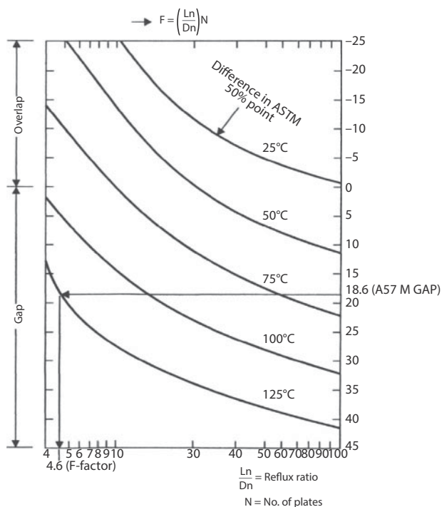
Figure 5.17 F-factor and ASTM gaps [8].
