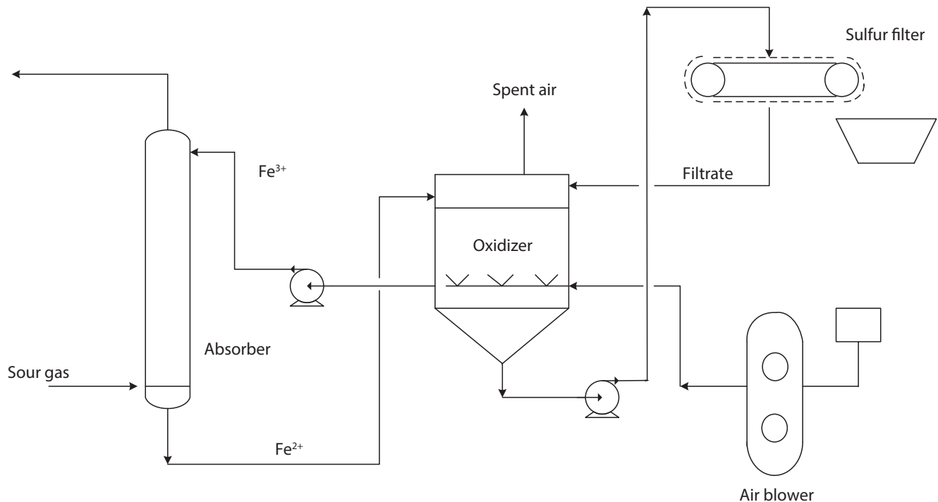
Figure 12.10 H 2 S removal process.
