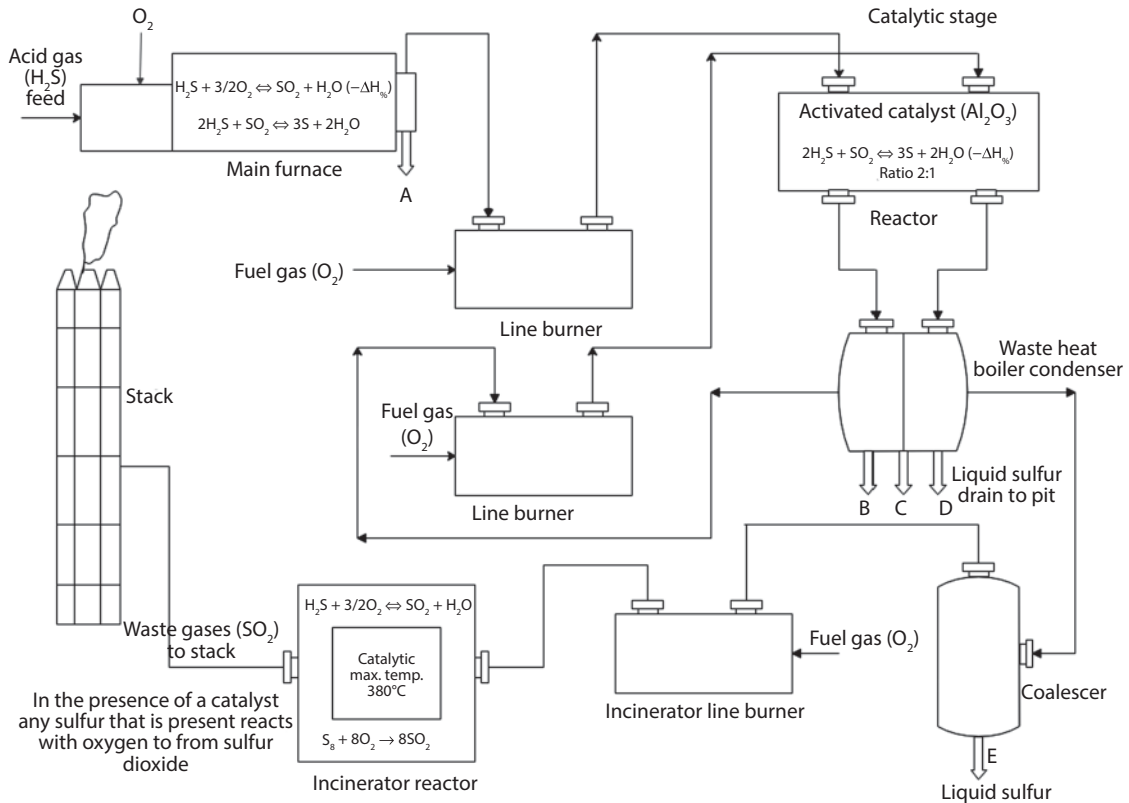
Figure 12.9 Sulfur recovery unit.
