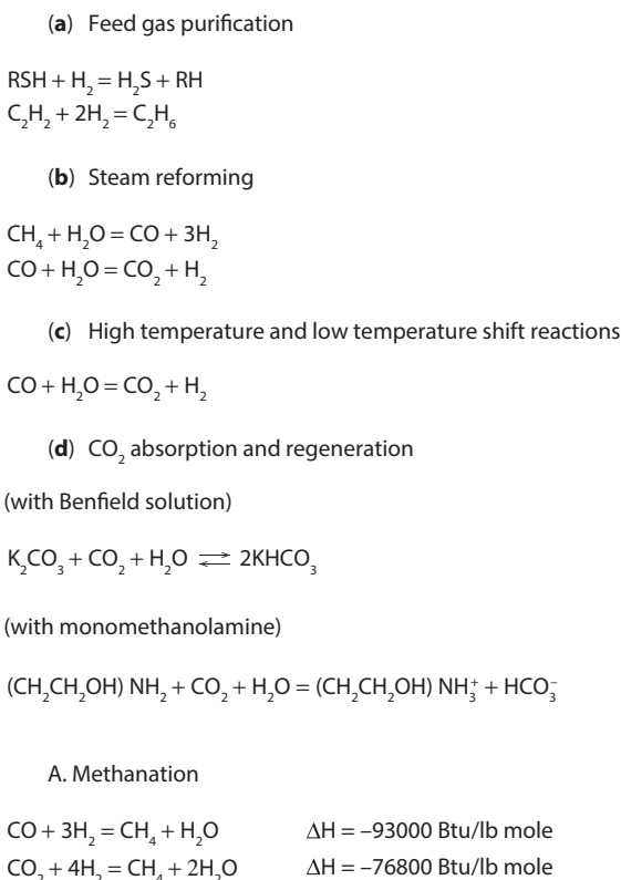
Figure 11.3 Chemical reactions involved in hydrogen production.
