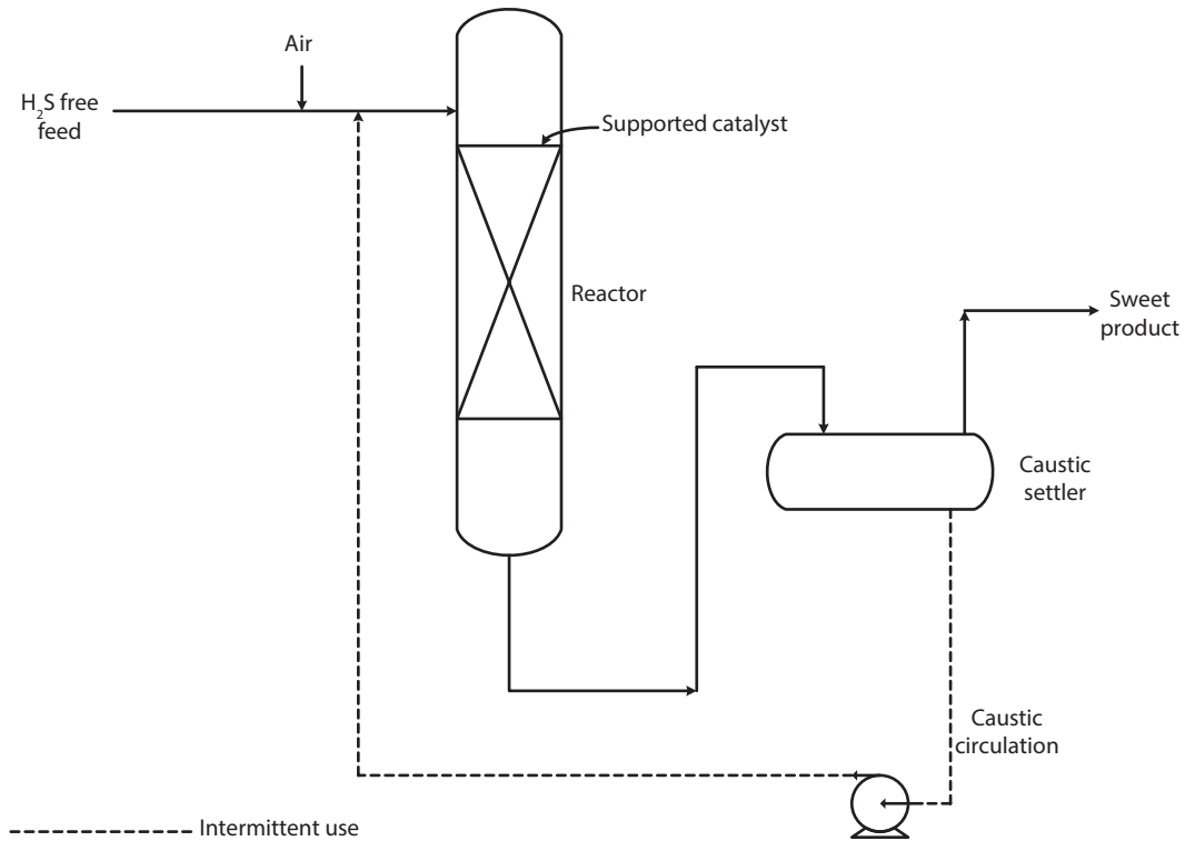
Figure 12.8 Fixed-bed Merox sweetening unit.
