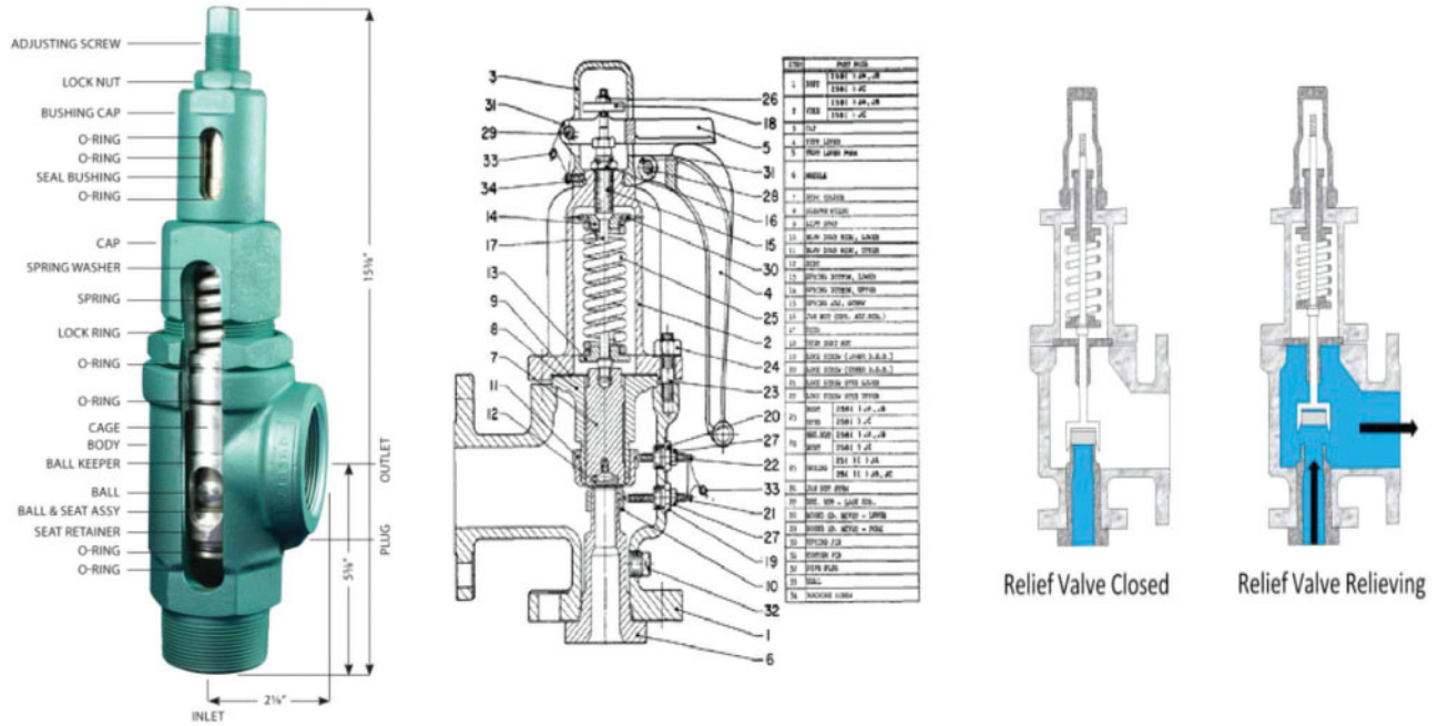
Figure 43 Relief valves.
