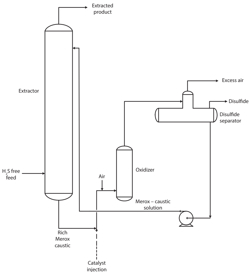
Figure 12.7 Flow diagram of Merox mercaptan-extraction unit.
