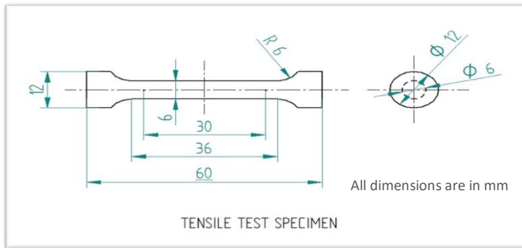
Fig.3.7.1: Tensile testing specimen
