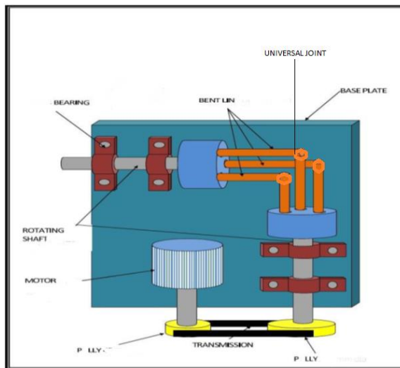
Fig-1: Concept Drawing of Machine
